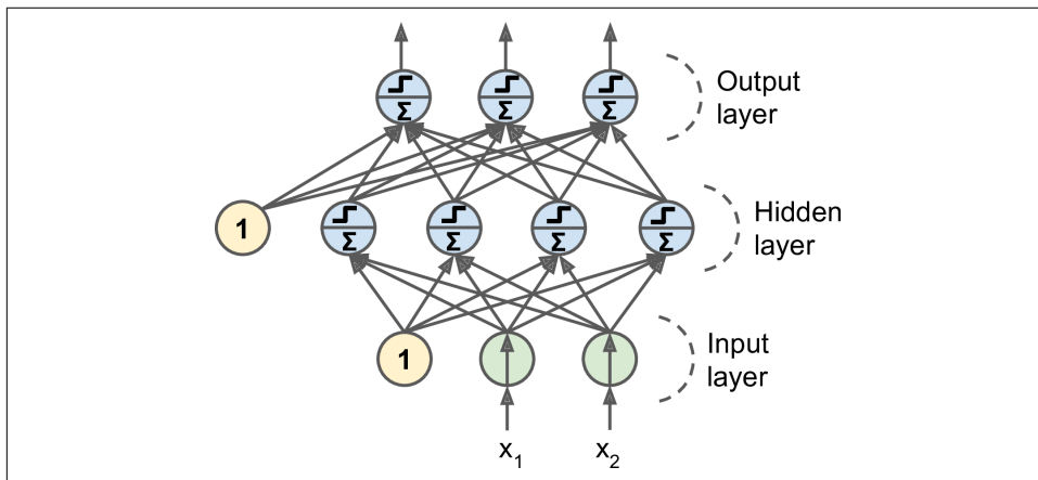
Figure 10-7. Multi-Layer Perceptron
