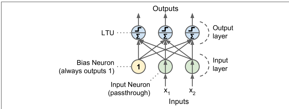
Figure 10-5. Perceptron diagram
