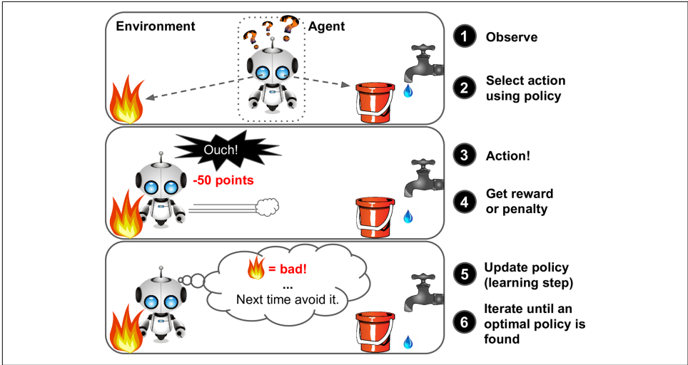
Figure 1-12. Reinforcement Learning
