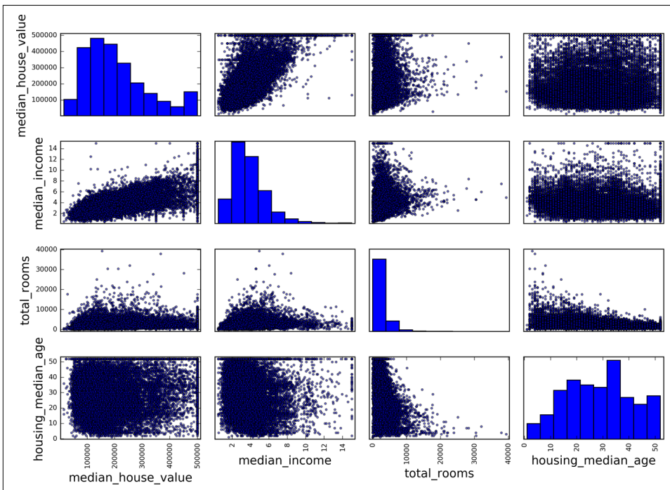
Figure 2-15. Scatter matrix
